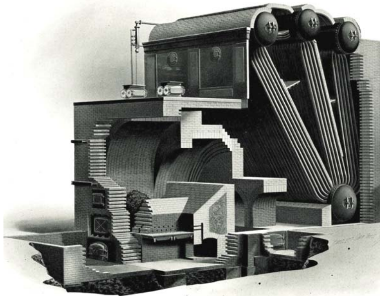
STIRLING BOILER SET WITH FURNACE FOR BURNING GREEN BAGASSE
